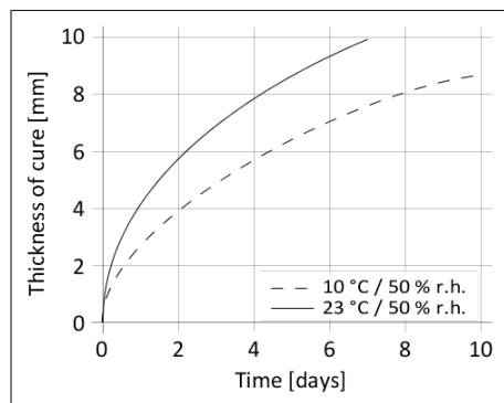
Diagram 1: Curing speed of Sikaflex®-265
